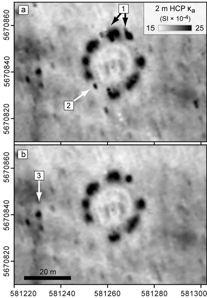
Fig. 5. Comparison of the anomalies detected at the hengiform monument (see Gaffney et al., 2012) as seen in the 2 m HCP k_a data before (a) and after (b) metal removal. In (a), two anomalies are indicated that were related to the metal topsoil debris, in (b) a group of anomalies are indicated that remained present in the filtered data, which suggest the presence of pits.
