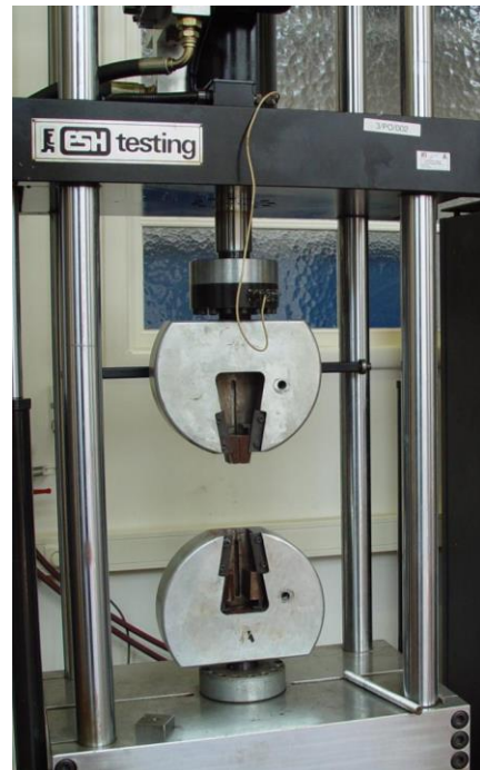
Figure 2: Medium Wide Plate tension test
