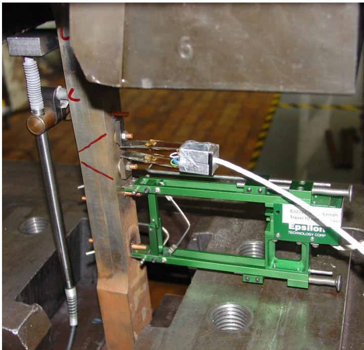
Figure 1: 8000 kN test rig
